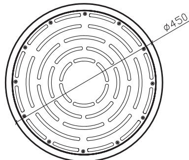
Tumbler base Bottom view
